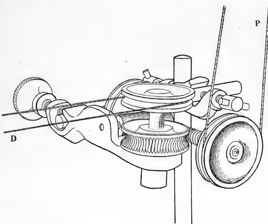
TEXT-FIG. 43. Reducing gear clamp attached to vertical standard for table-bench. P, the power-cord; D, the distributing-cord moving eighty times more slowly than P.
